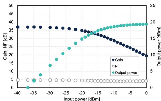
Gain/NF/output power vs. input power @1550nm
