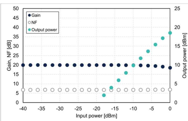
Gain/NF/output power vs. input power @1620nm
