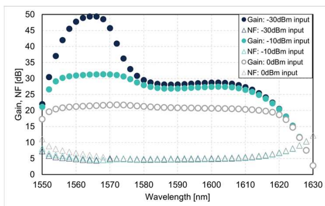
Gain/noise figure vs. wavelength
