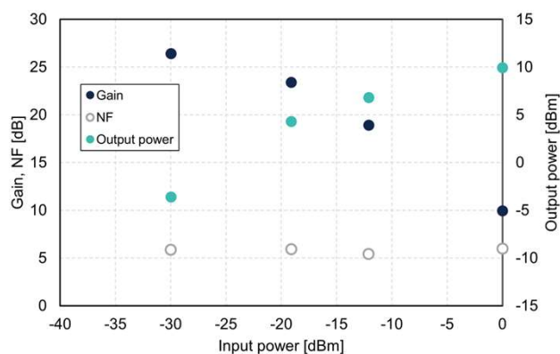
Gain/NF/output power vs. input power @850nm
