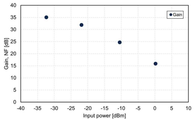
Gain/NF/output power vs. input power @980nm
