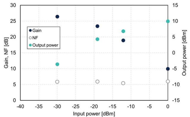
Gain/NF/output power vs. input power @850nm
