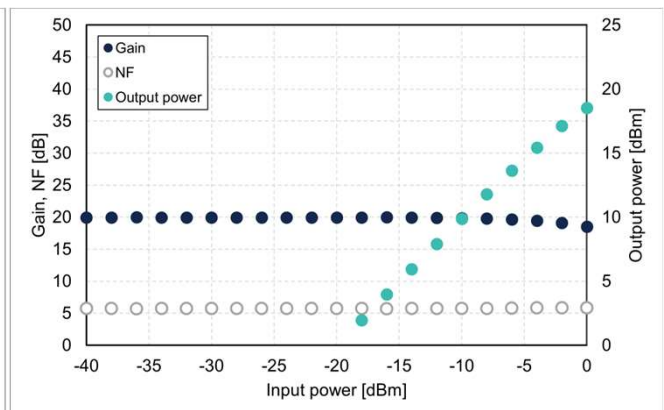
Gain/NF/output power vs. input power @1620nm
