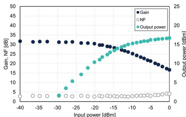
Gain/NF/output power vs. input power @1550nm
